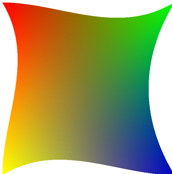
CoonsPatchMesh()
